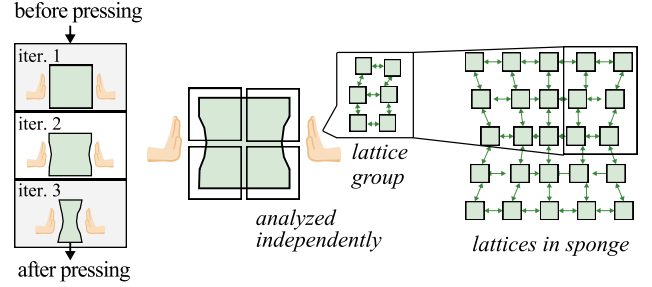
(a) Modeling the deformation of a sponge under compression by FEM.
