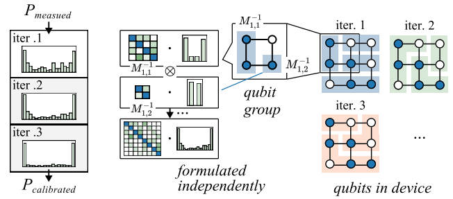
(b) Methodology of QuFEM inspired from FEM.
